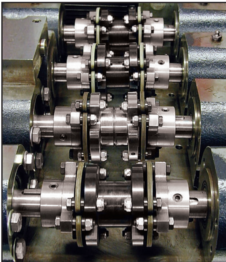
Floating Shaft Couplings on test in the Zero-Max test lab. This system is designed to run continuously at high misalignment, subjecting the composite unitized disc packs to billions of flexural fatigue cycles.
